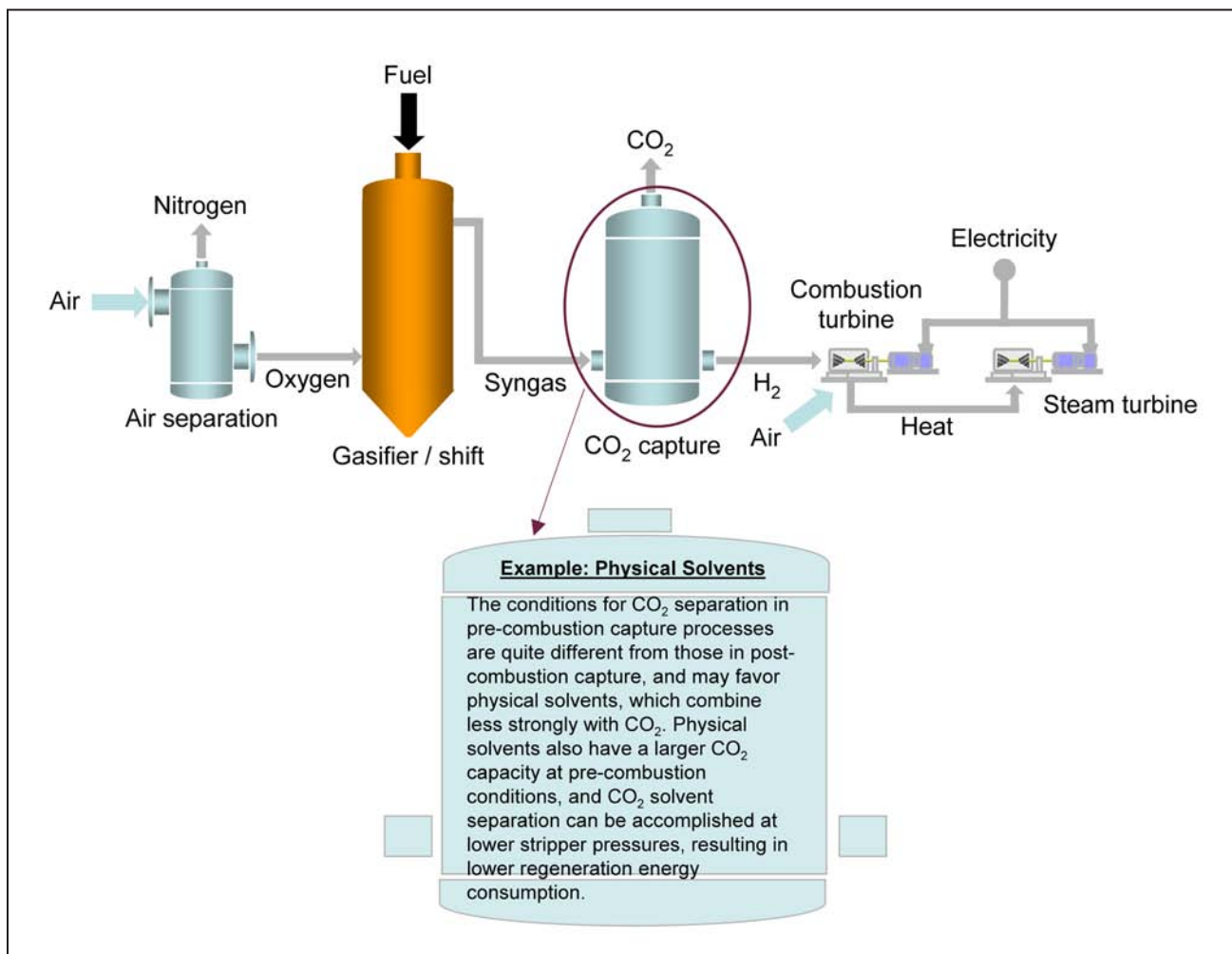
Figure 10. Pre-Combustion Capture
