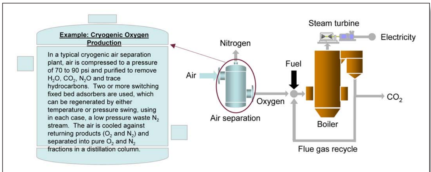
Figure 11. Oxy-Combustion
