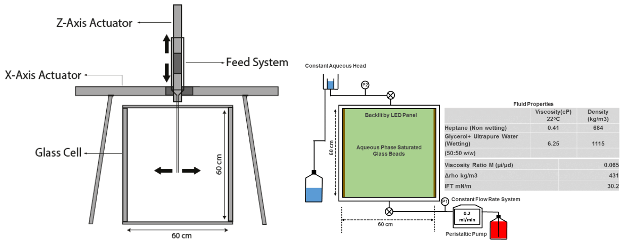
Fig 1: (LEFT) Schematic of the automated packing system, further developed from Griffith et al., 2013. (RIGHT) Setup for multi-phase buoyant flow experiments using surrogate fluids for subsurface conditions.
